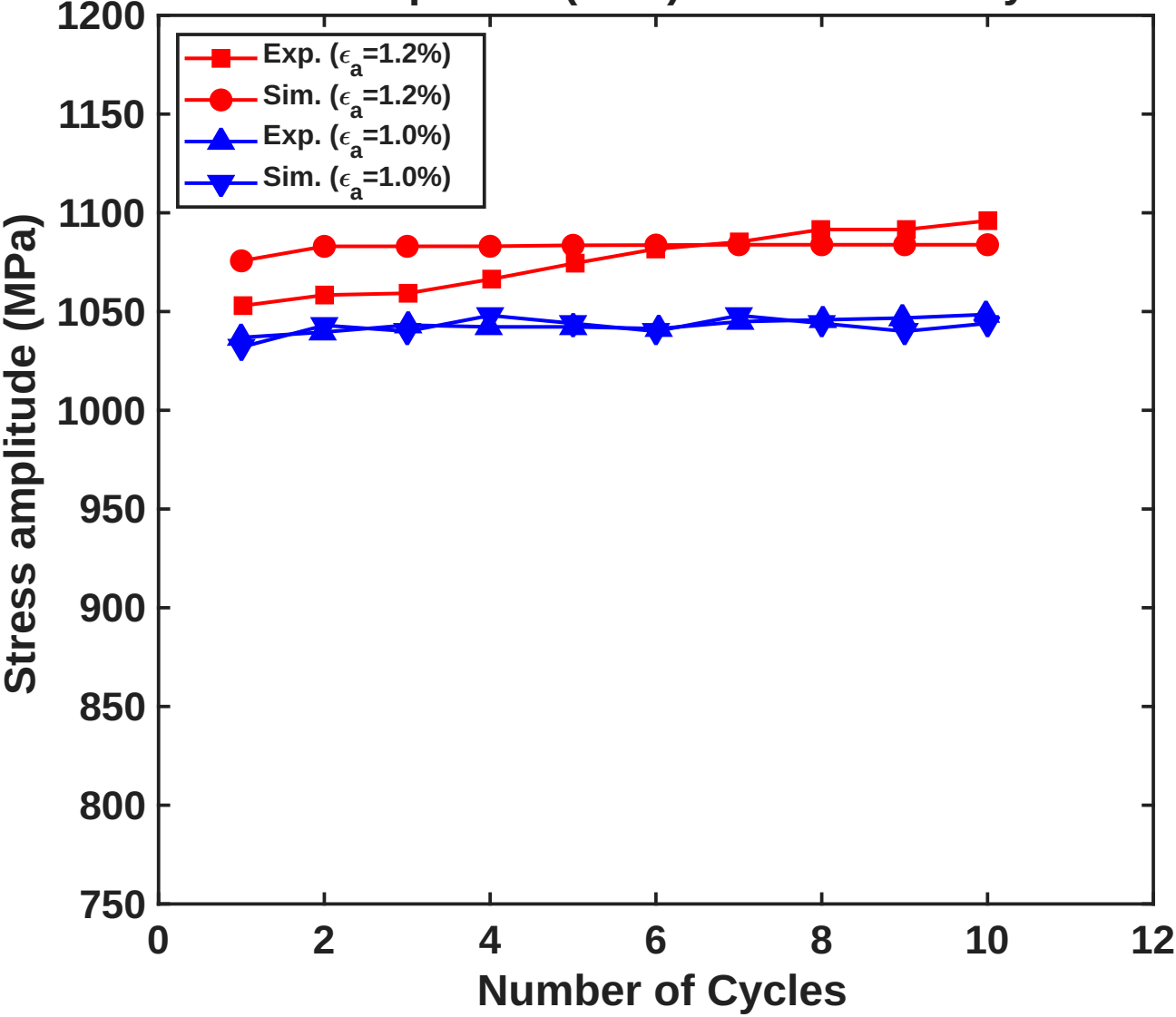
Stress amplitude (MPa) vs Number of Cycles
